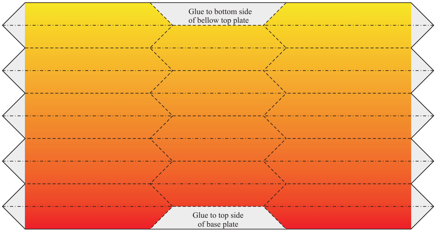
Bellow side wall
